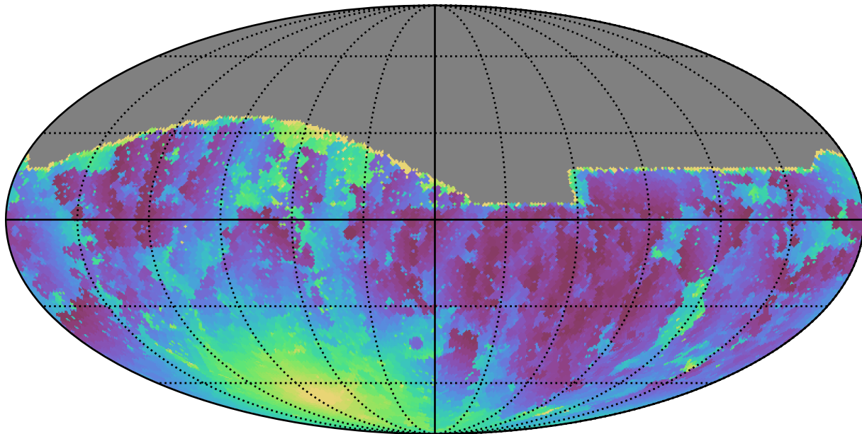
roll_pause_mjdp120_v3.4_10yrs All sky g band: Min moonDistance
