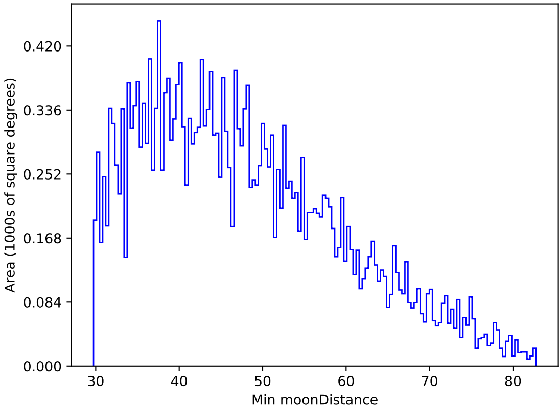
roll_pause_mjdp120_v3.4_10yrs All sky g band: Min moonDistance
