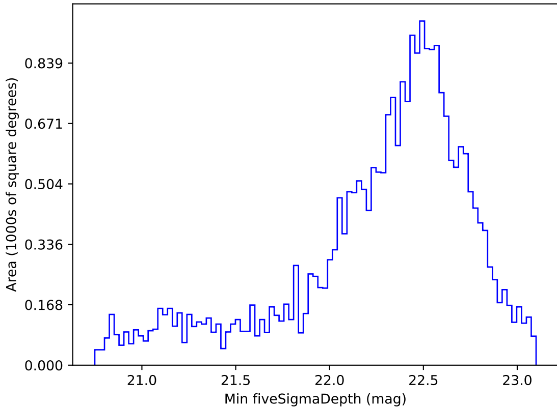
roll_pause_mjdp120_v3.4_10yrs Yr 1 z band: Min fiveSigmaDepth
