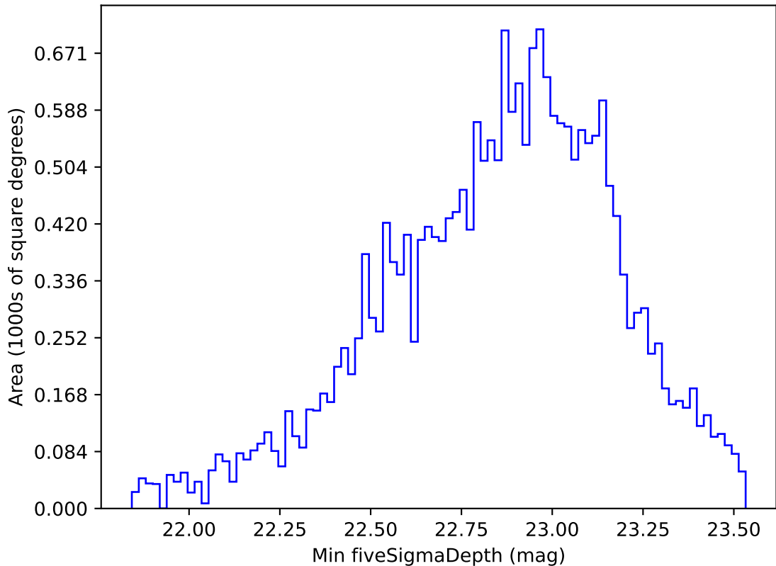
roll_pause_mjdp120_v3.4_10yrs Yr 1 u band: Min fiveSigmaDepth
