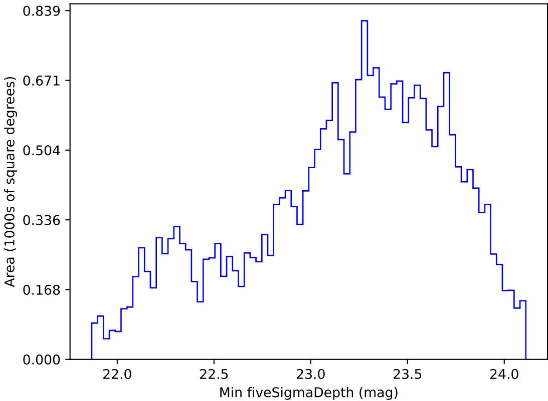
roll_pause_mjdp120_v3.4_10yrs Yr 1 r band: Min fiveSigmaDepth
