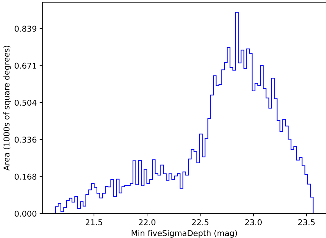
roll_pause_mjdp120_v3.4_10yrs Yr 1 i band: Min fiveSigmaDepth
