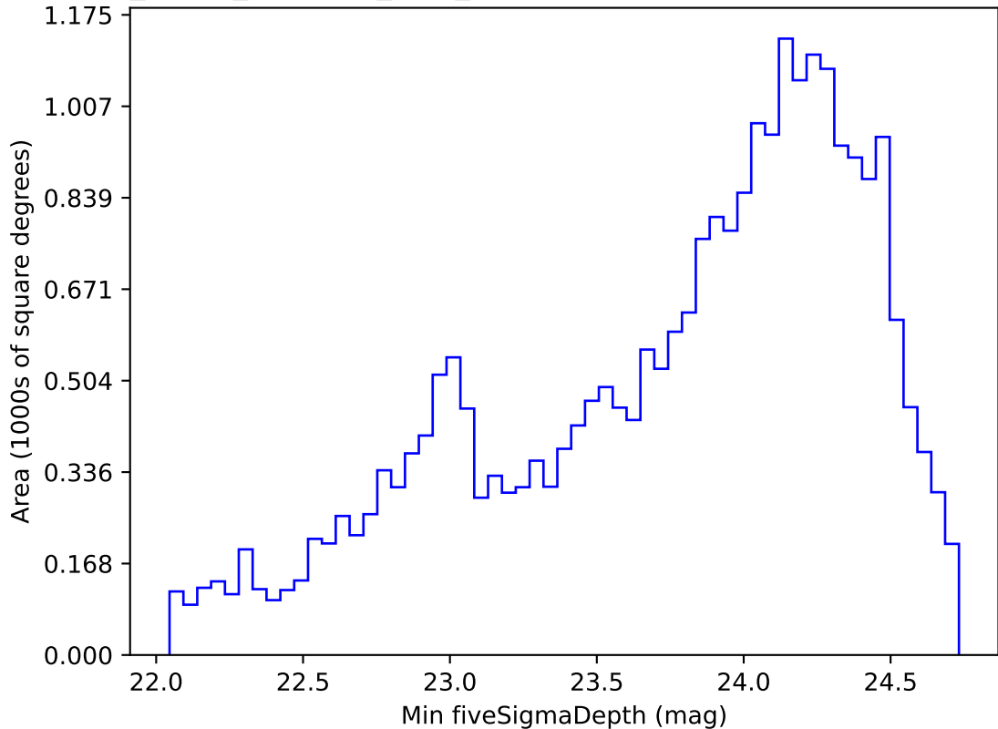
roll_pause_mjdp120_v3.4_10yrs Yr 1 g band: Min fiveSigmaDepth
