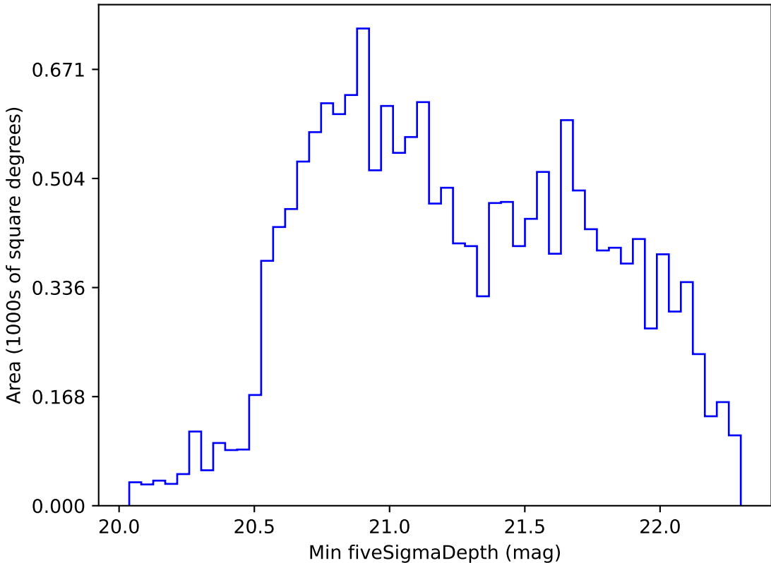
roll_pause_mjdp120_v3.4_10yrs WFD z band: Min fiveSigmaDepth
