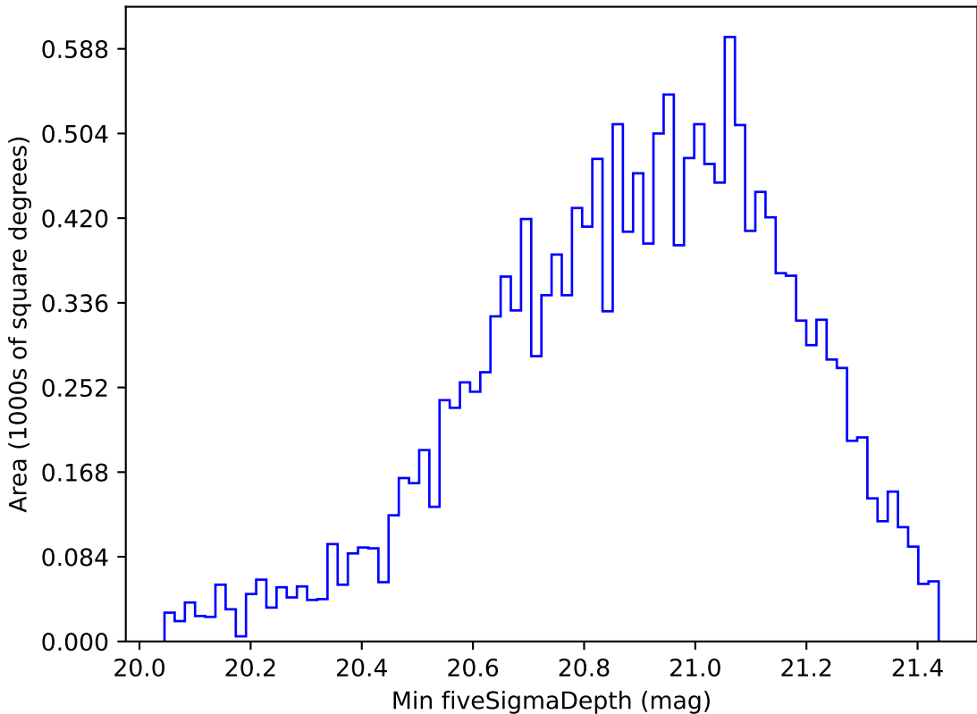
roll_pause_mjdp120_v3.4_10yrs WFD y band: Min fiveSigmaDepth
