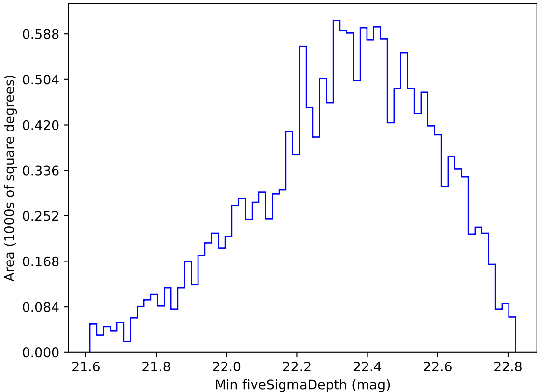
roll_pause_mjdp120_v3.4_10yrs WFD u band: Min fiveSigmaDepth
