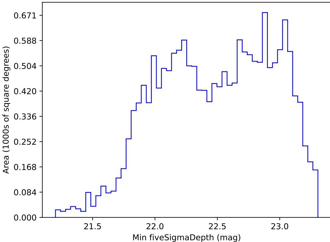
roll_pause_mjdp120_v3.4_10yrs WFD r band: Min fiveSigmaDepth
