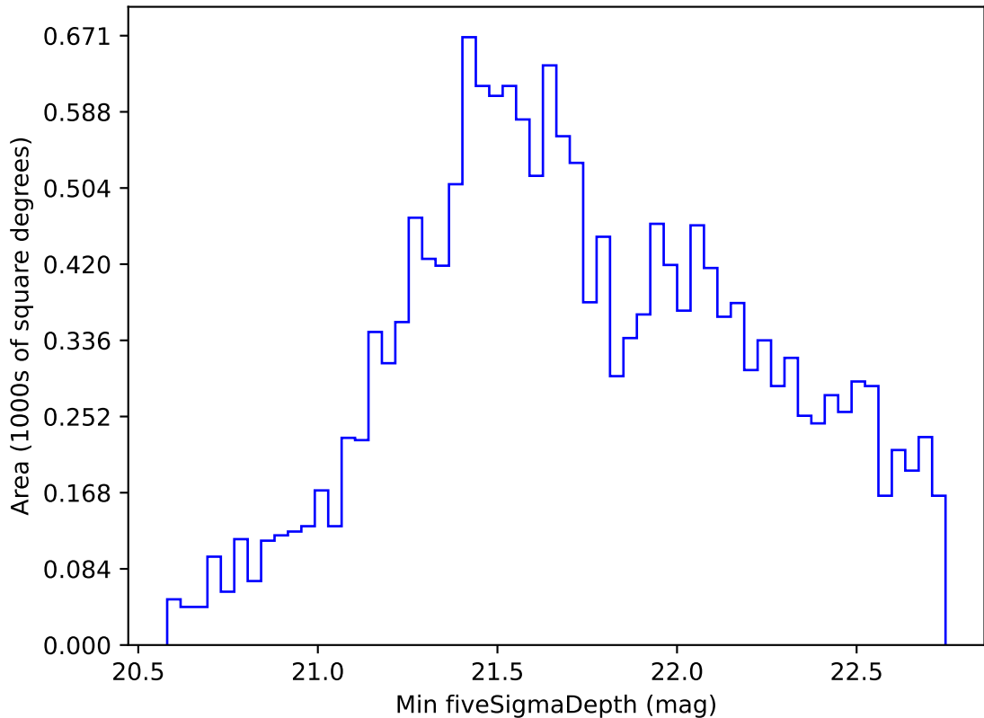
roll_pause_mjdp120_v3.4_10yrs WFD i band: Min fiveSigmaDepth
