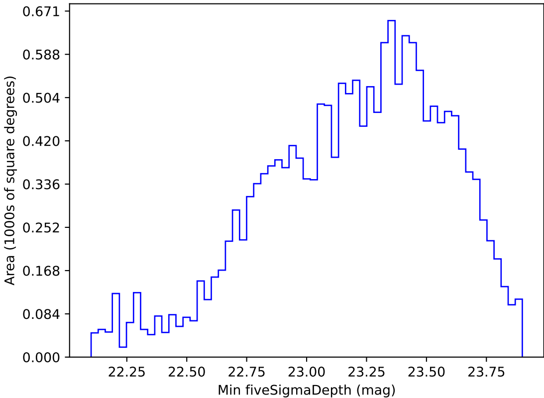
roll_pause_mjdp120_v3.4_10yrs WFD g band: Min fiveSigmaDepth
