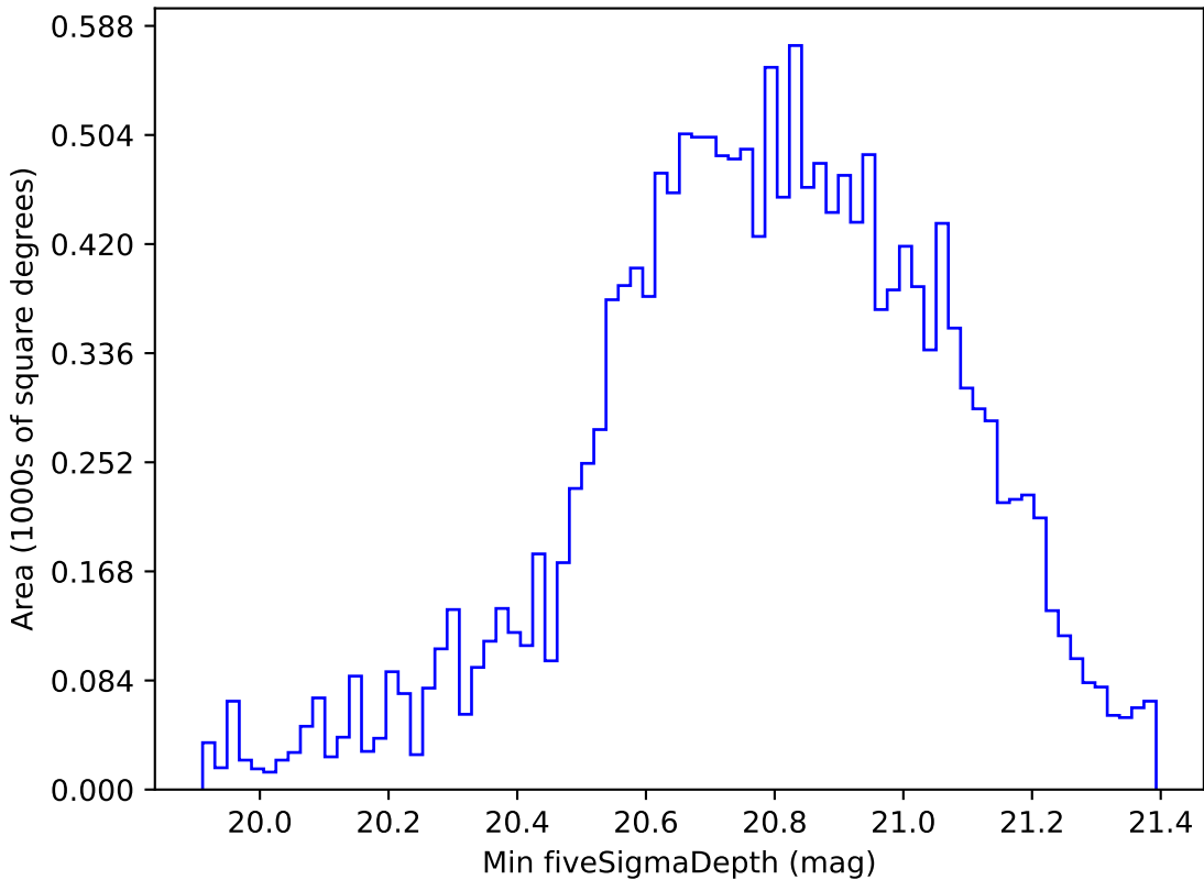
roll_pause_mjdp120_v3.4_10yrs WFD all bands: Min fiveSigmaDepth
