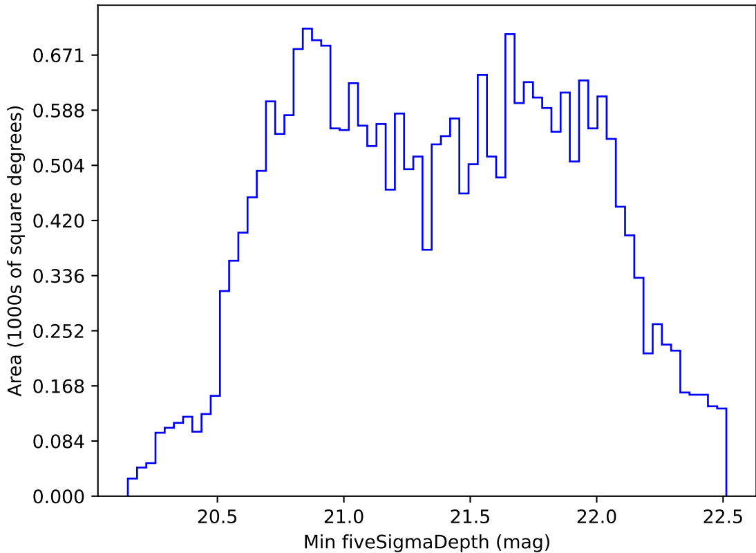
roll_pause_mjdp120_v3.4_10yrs All sky z band: Min fiveSigmaDepth
