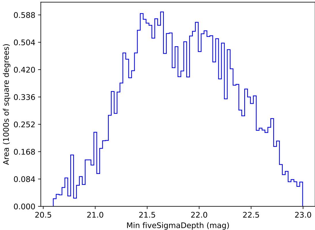
roll_pause_mjdp120_v3.4_10yrs All sky i band: Min fiveSigmaDepth
