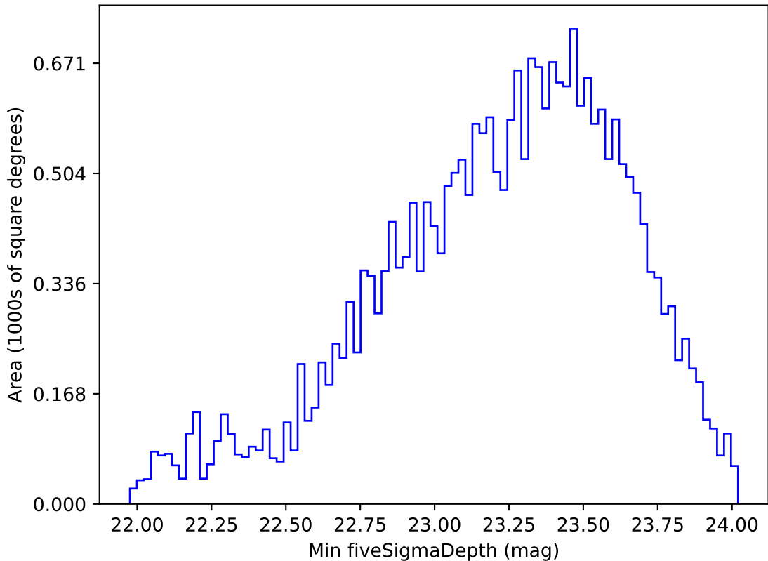
roll_pause_mjdp120_v3.4_10yrs All sky g band: Min fiveSigmaDepth
