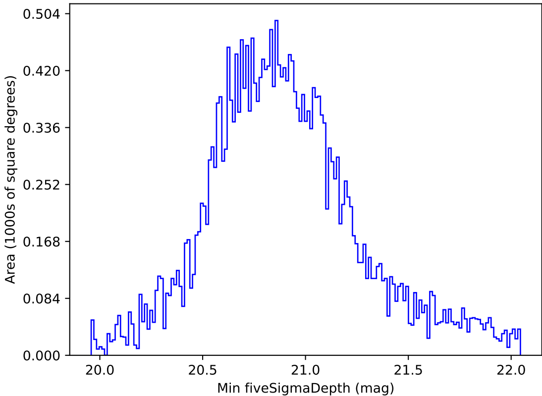
roll_pause_mjdp120_v3.4_10yrs All sky all bands: Min fiveSigmaDepth
