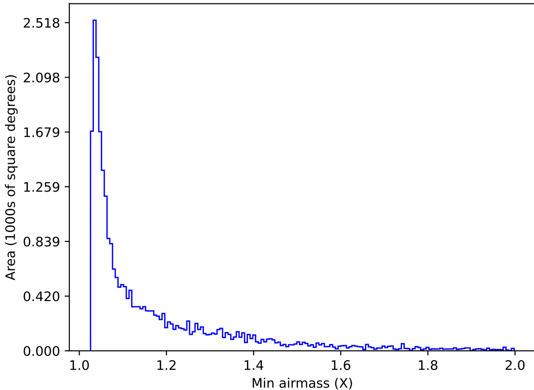
roll_pause_mjdp120_v3.4_10yrs Yr 1 z band: Min airmass
