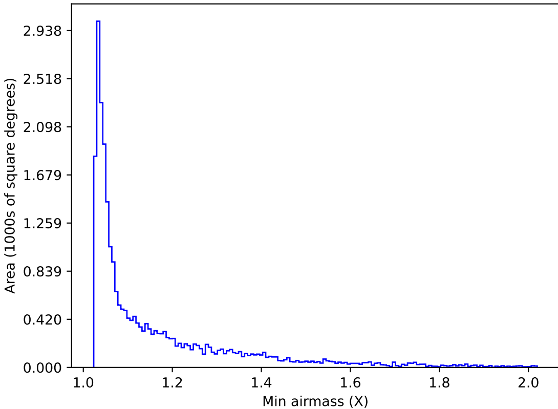
roll_pause_mjdp120_v3.4_10yrs Yr 1 r band: Min airmass
