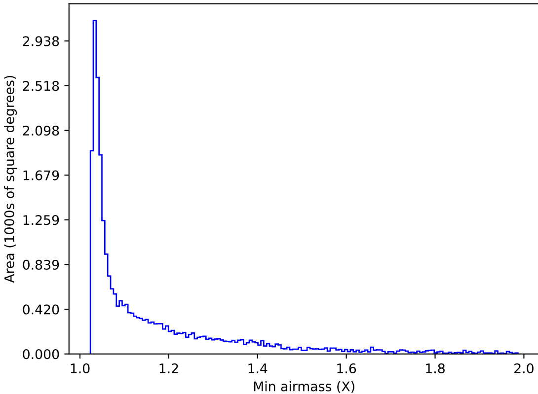
roll_pause_mjdp120_v3.4_10yrs Yr 1 i band: Min airmass
