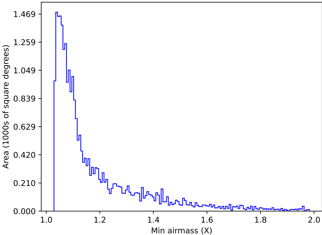
roll_pause_mjdp120_v3.4_10yrs Yr 1 g band: Min airmass
