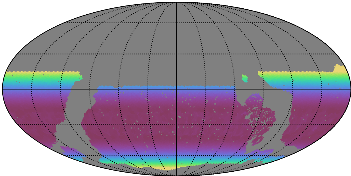
roll_pause_mjdp120_v3.4_10yrs WFD z band: Min airmass
