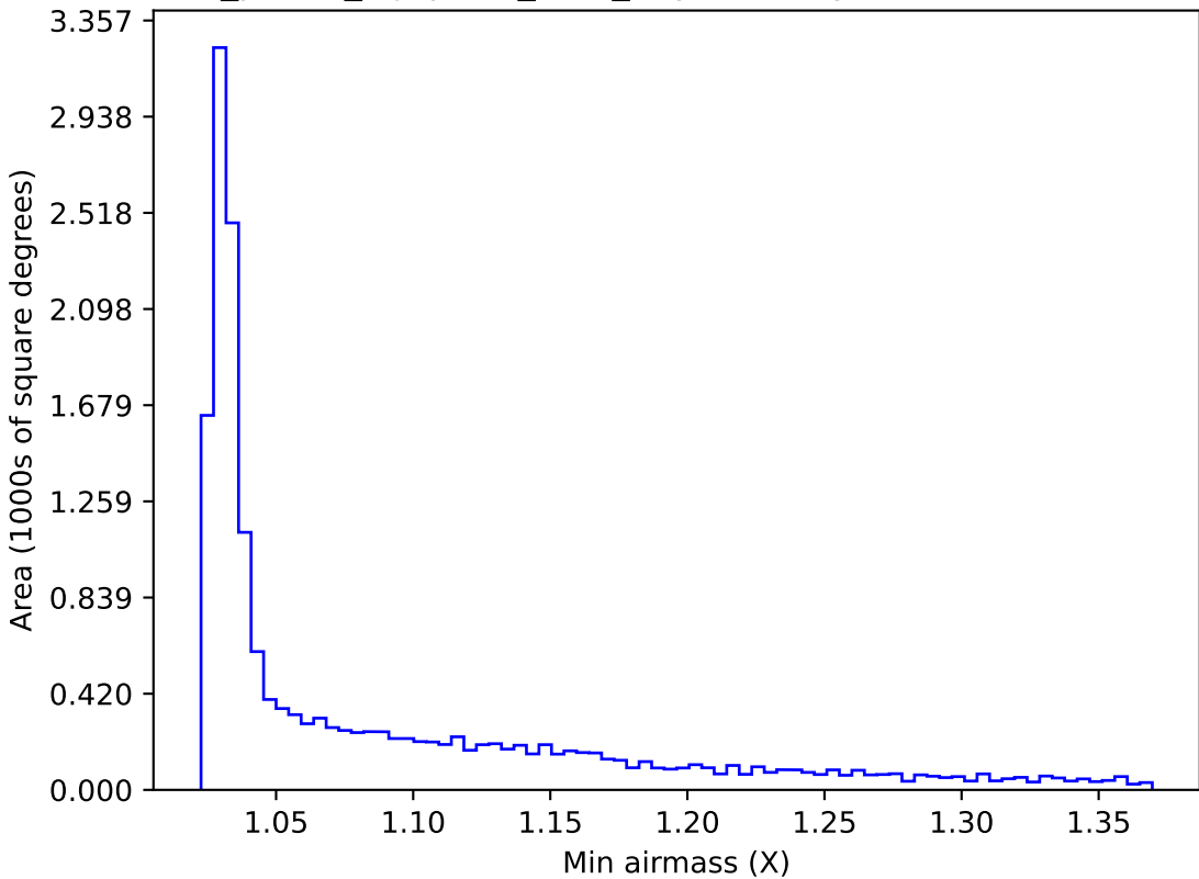
roll_pause_mjdp120_v3.4_10yrs WFD y band: Min airmass
