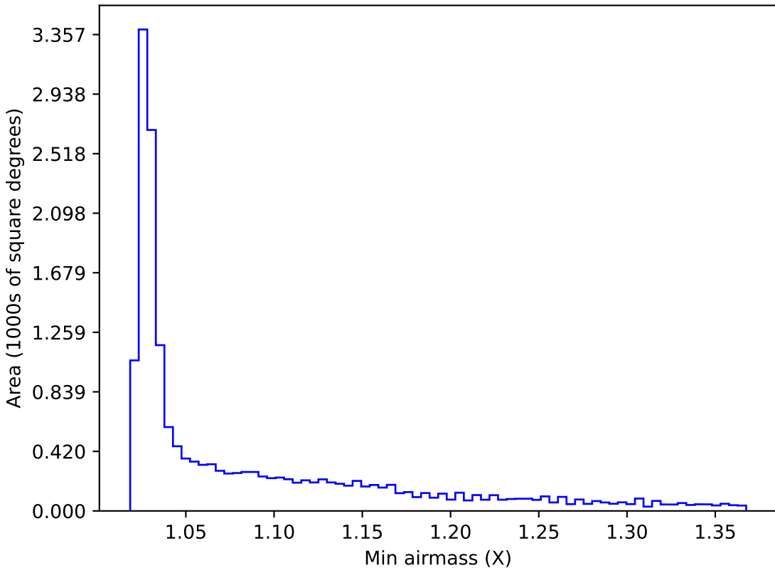
roll_pause_mjdp120_v3.4_10yrs WFD i band: Min airmass
