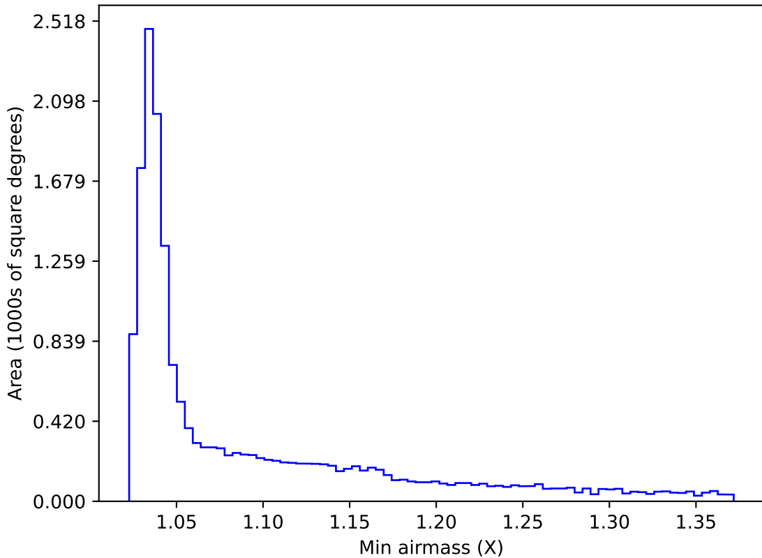
roll_pause_mjdp120_v3.4_10yrs WFD g band: Min airmass
