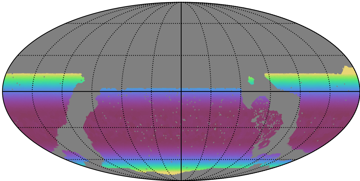
roll_pause_mjdp120_v3.4_10yrs WFD all bands: Min airmass
