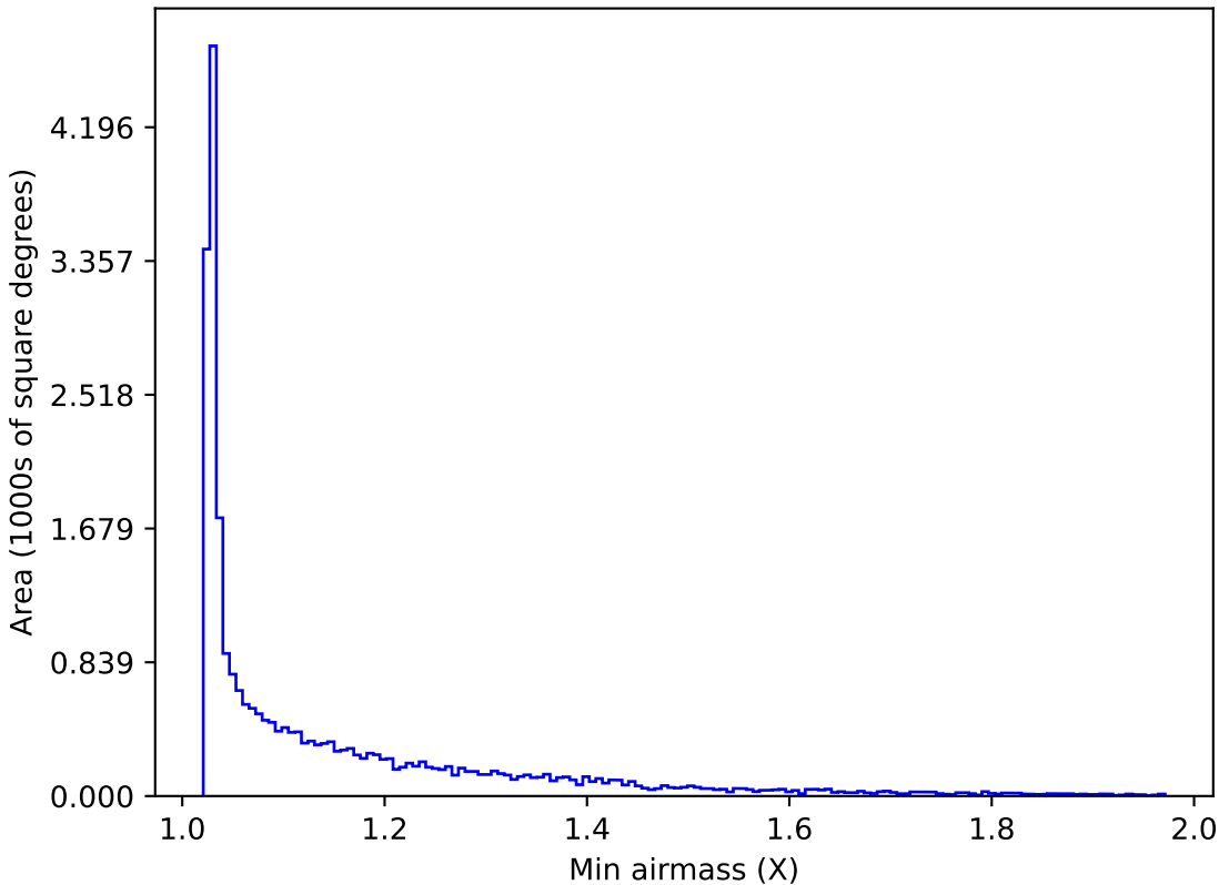
roll_pause_mjdp120_v3.4_10yrs All sky z band: Min airmass
