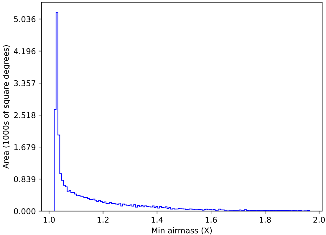
roll_pause_mjdp120_v3.4_10yrs All sky i band: Min airmass
