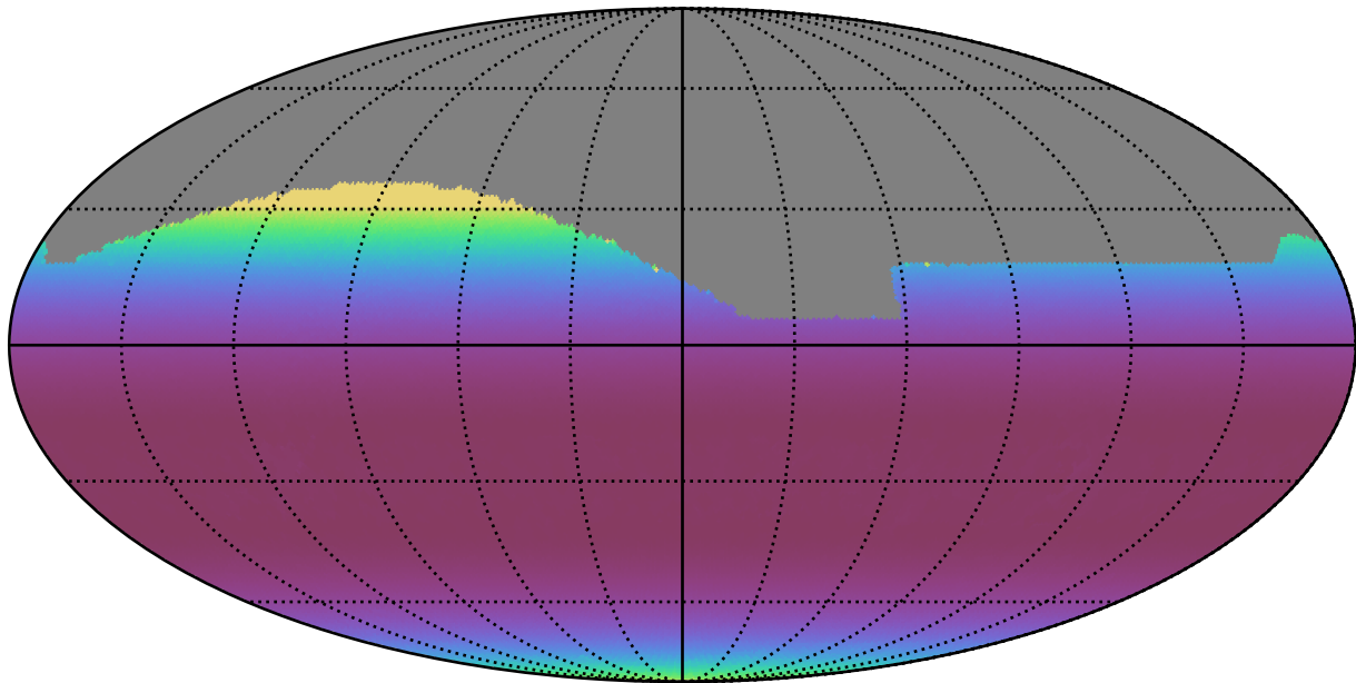
roll_pause_mjdp120_v3.4_10yrs All sky all bands: Min airmass
