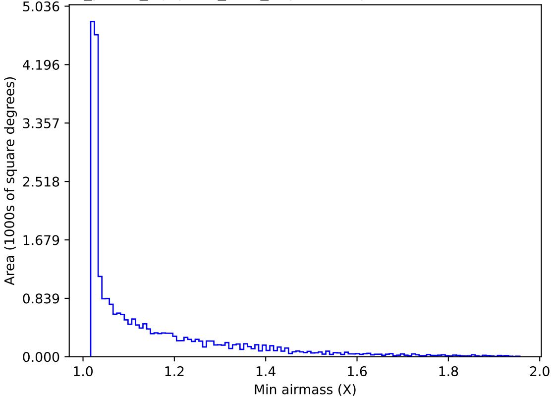
roll_pause_mjdp120_v3.4_10yrs All sky all bands: Min airmass
