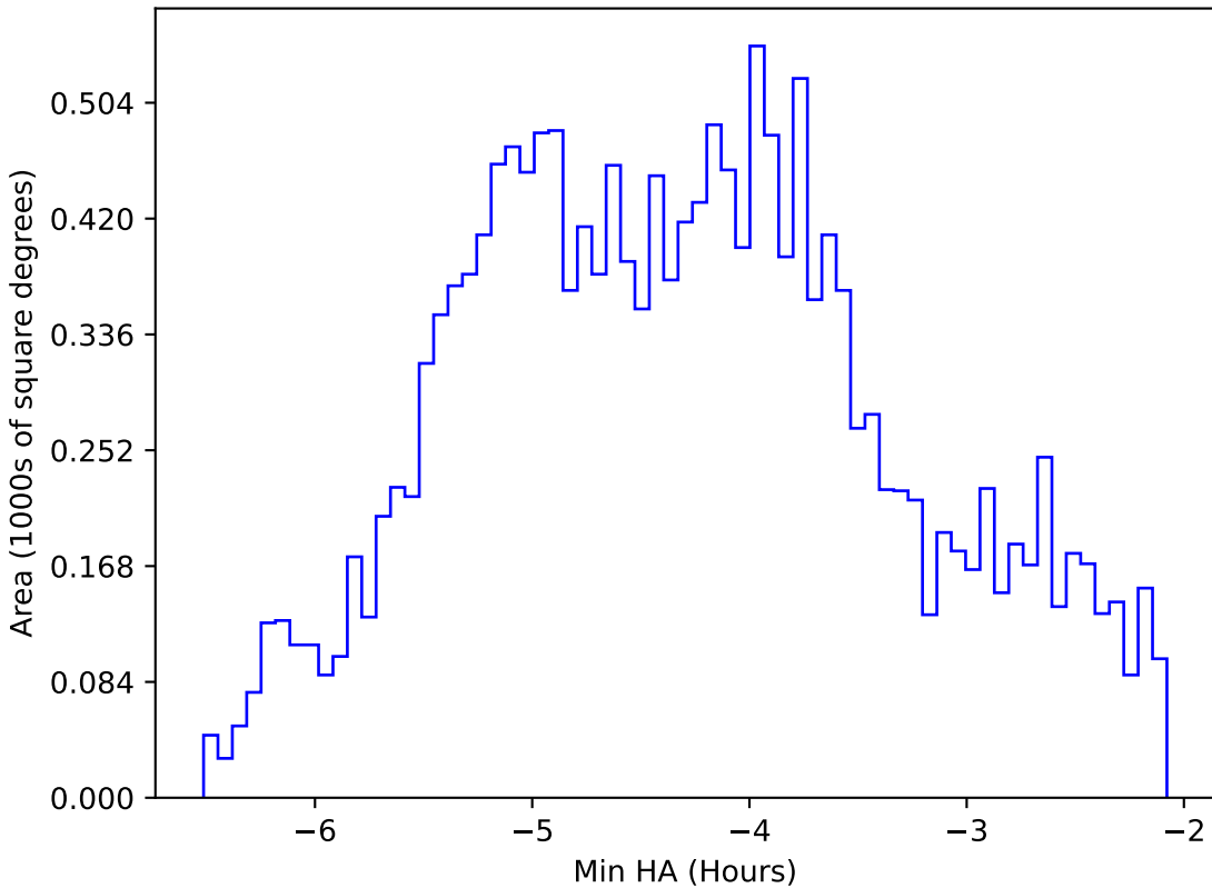
roll_pause_mjdp120_v3.4_10yrs WFD z band: Min HA
