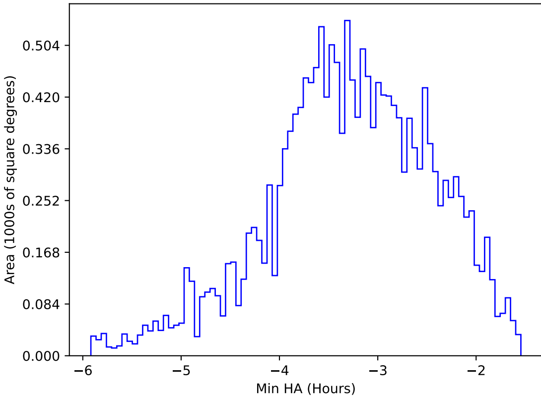
roll_pause_mjdp120_v3.4_10yrs WFD u band: Min HA
