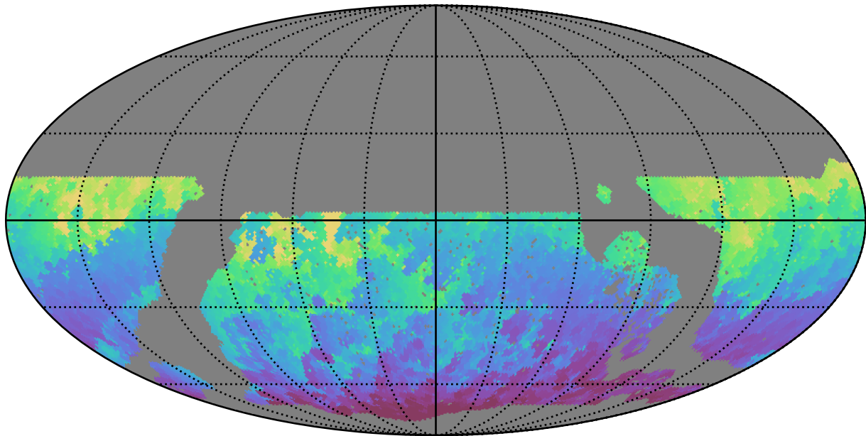
roll_pause_mjdp120_v3.4_10yrs WFD i band: Min HA
