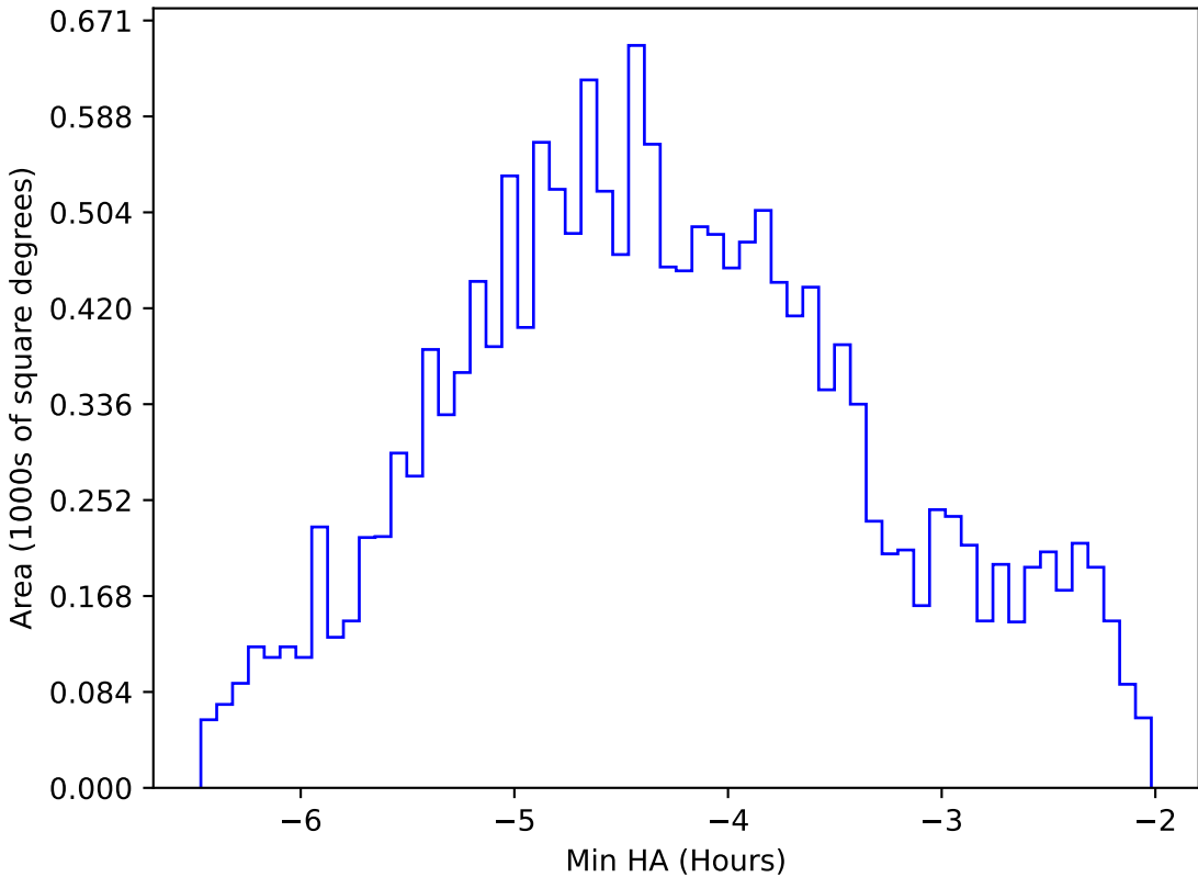
roll_pause_mjdp120_v3.4_10yrs WFD i band: Min HA
