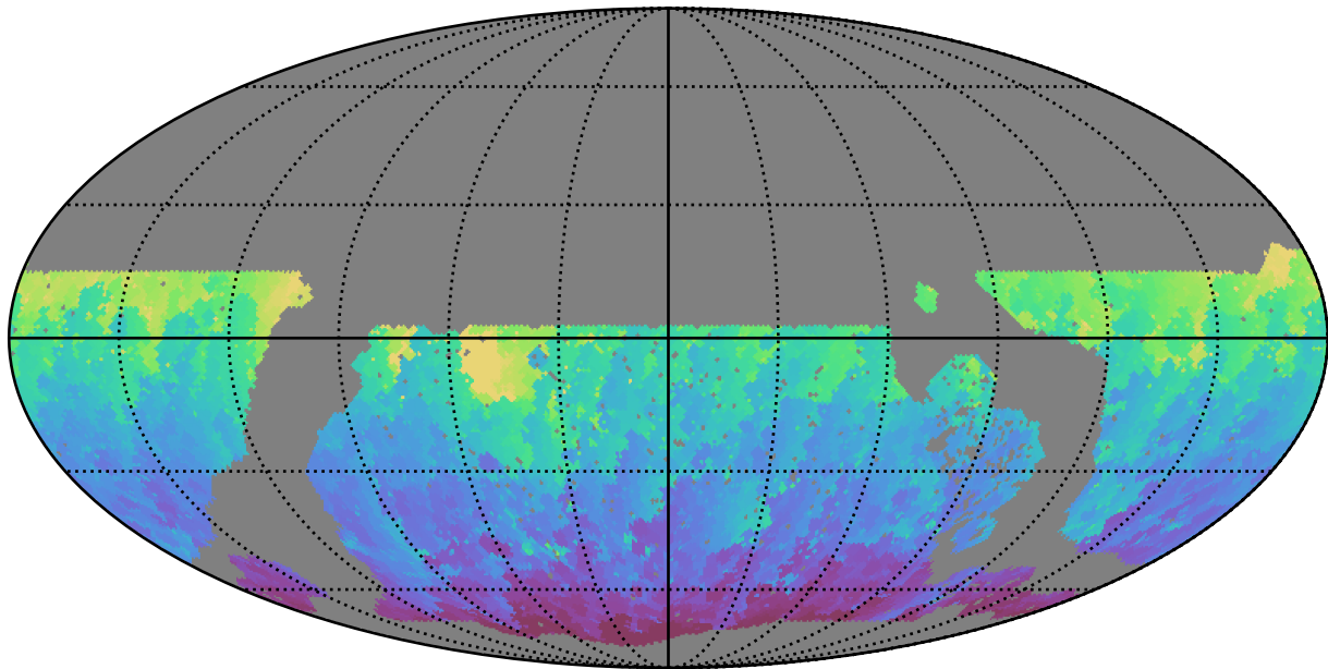
roll_pause_mjdp120_v3.4_10yrs WFD g band: Min HA
