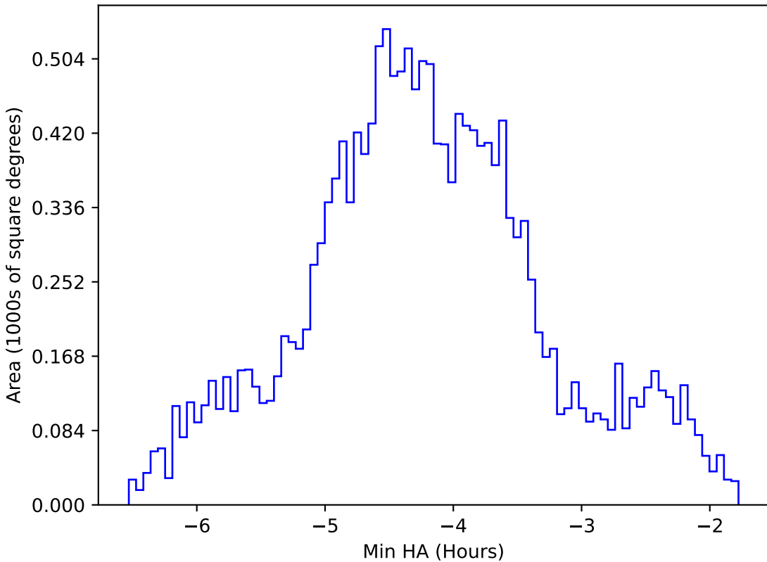
roll_pause_mjdp120_v3.4_10yrs WFD g band: Min HA
