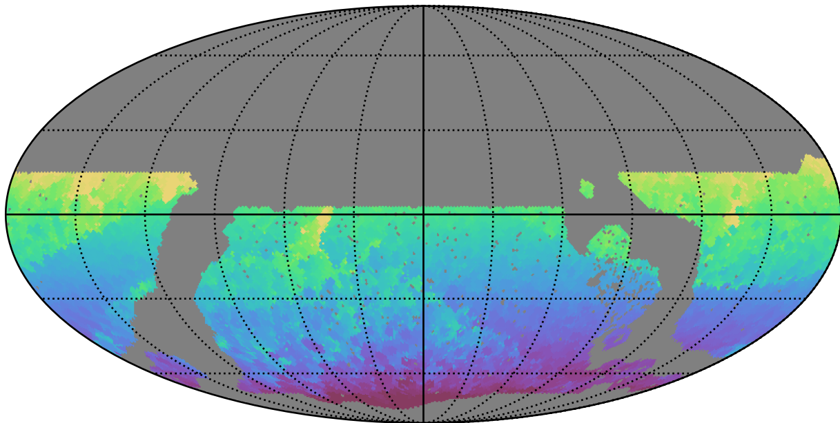
roll_pause_mjdp120_v3.4_10yrs WFD all bands: Min HA
