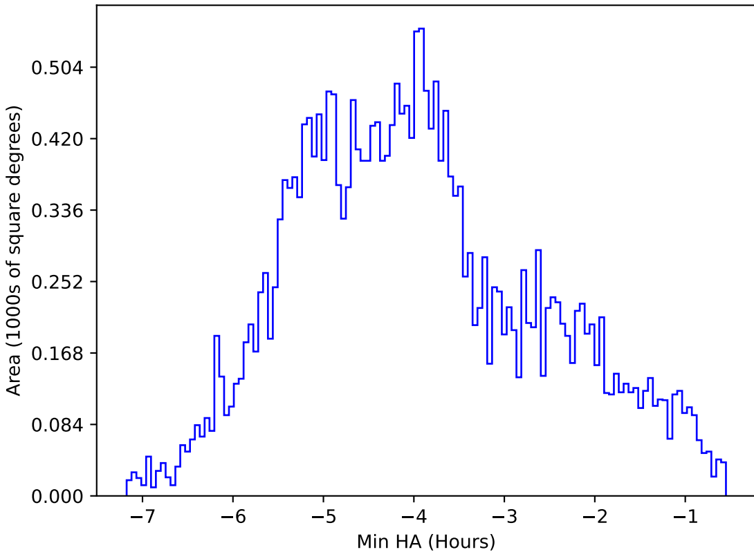
roll_pause_mjdp120_v3.4_10yrs All sky z band: Min HA
