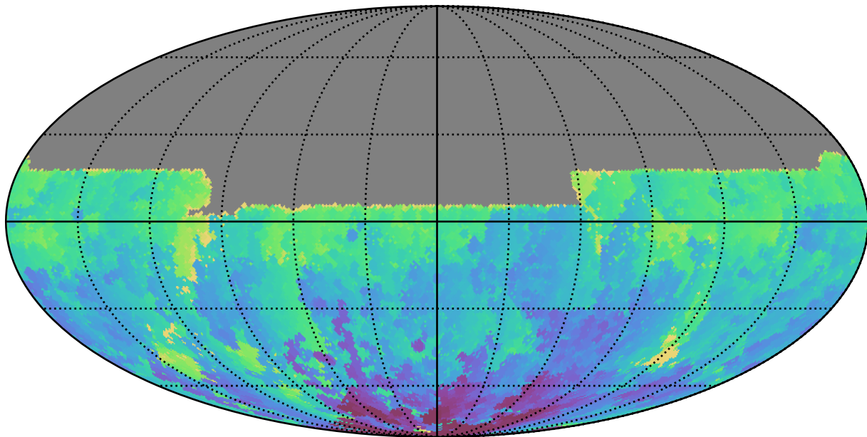
roll_pause_mjdp120_v3.4_10yrs All sky u band: Min HA
