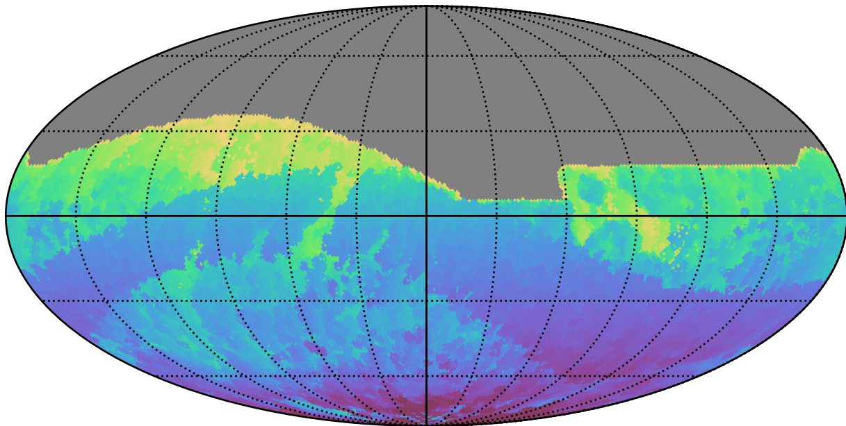
roll_pause_mjdp120_v3.4_10yrs All sky r band: Min HA
