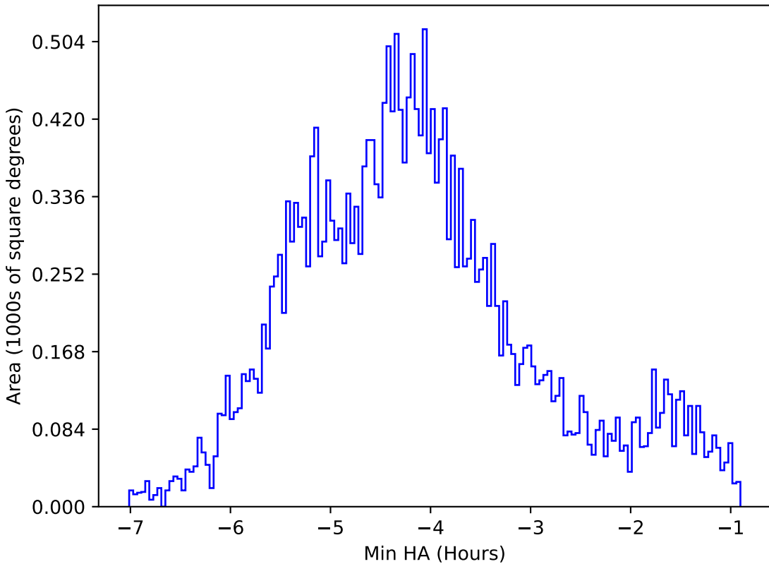
roll_pause_mjdp120_v3.4_10yrs All sky r band: Min HA
