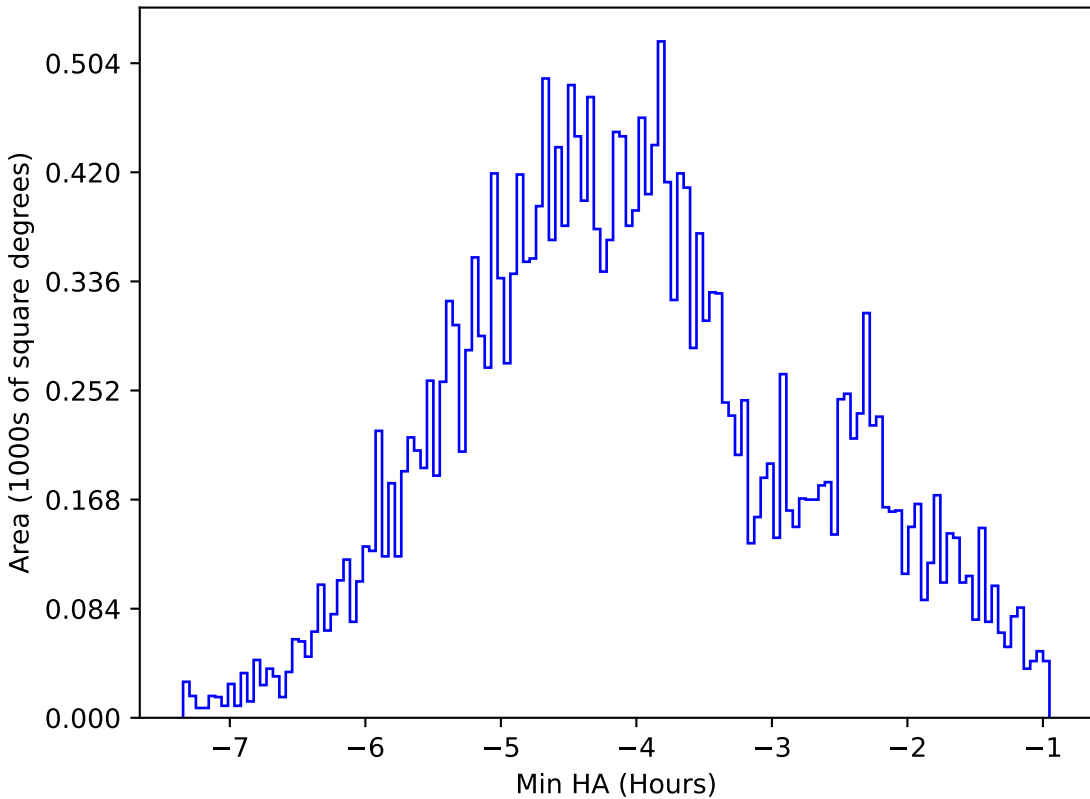
roll_pause_mjdp120_v3.4_10yrs All sky i band: Min HA
