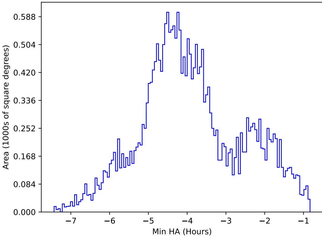
roll_pause_mjdp120_v3.4_10yrs All sky g band: Min HA
