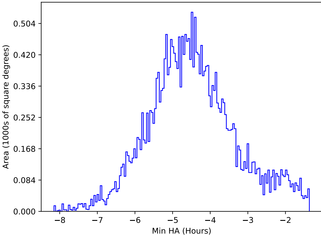
roll_pause_mjdp120_v3.4_10yrs All sky all bands: Min HA
