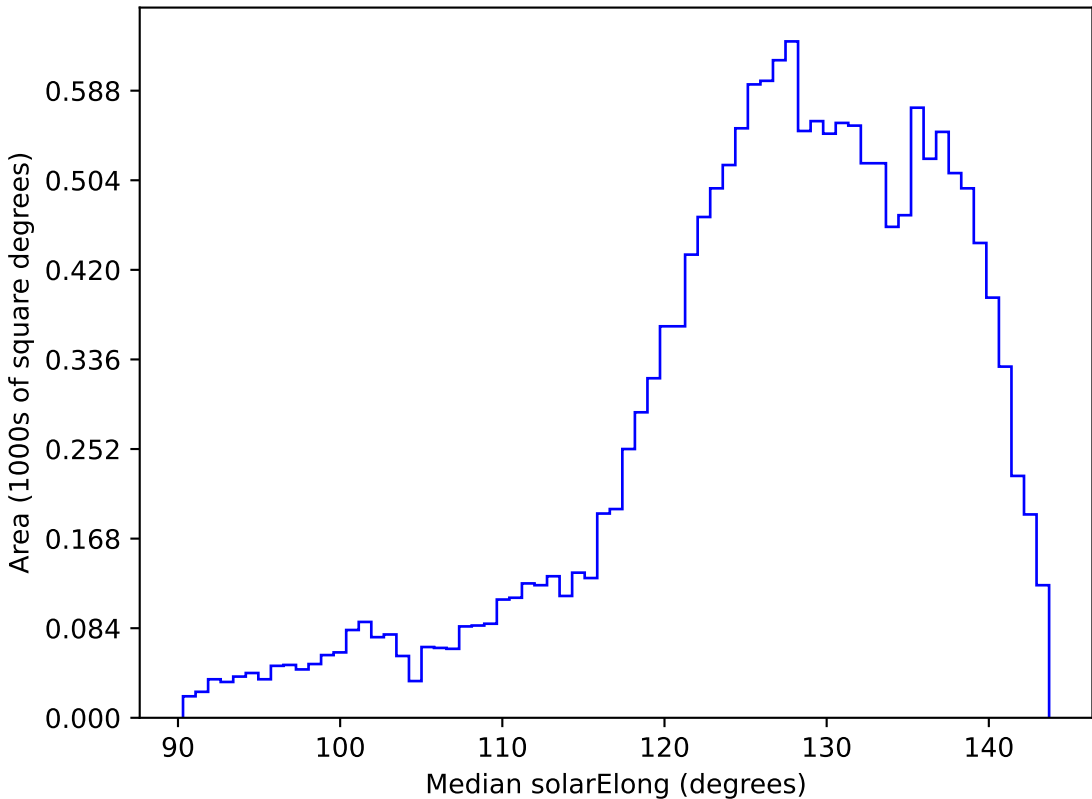
roll_pause_mjdp120_v3.4_10yrs WFD z band: Median solarElong
