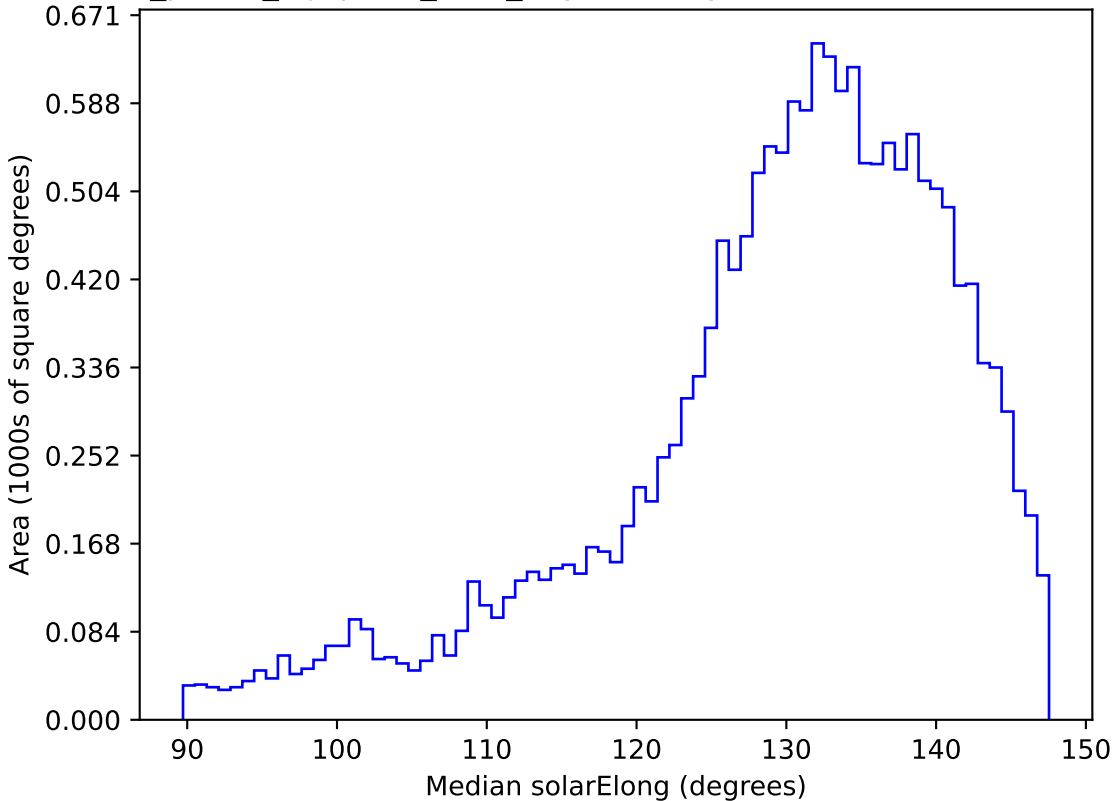
roll_pause_mjdp120_v3.4_10yrs WFD y band: Median solarElong
