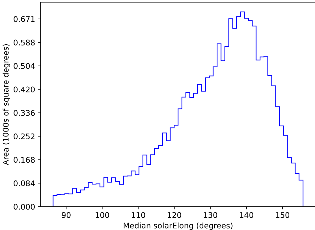
roll_pause_mjdp120_v3.4_10yrs WFD u band: Median solarElong
