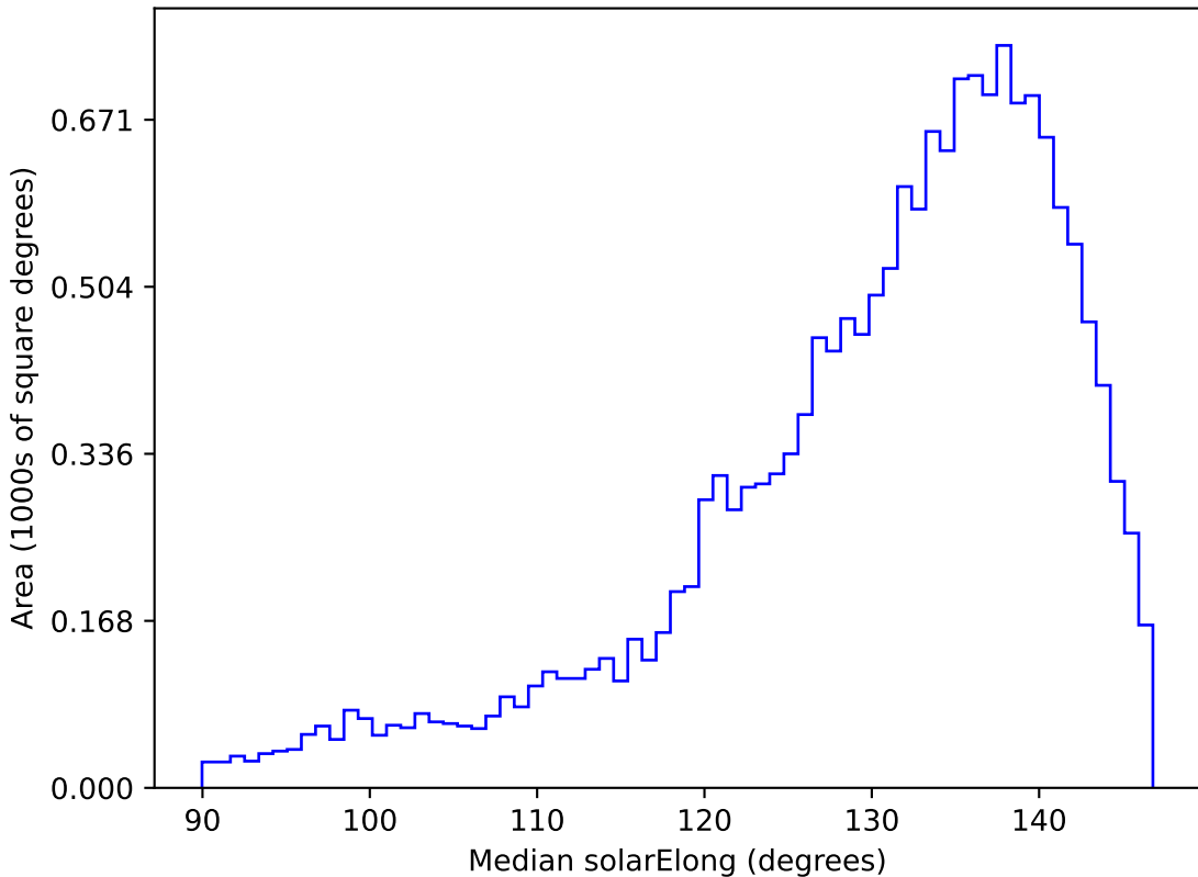
roll_pause_mjdp120_v3.4_10yrs WFD r band: Median solarElong
