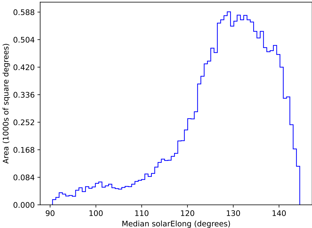
roll_pause_mjdp120_v3.4_10yrs WFD i band: Median solarElong
